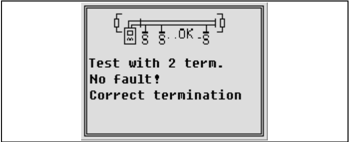
Figure 10: Screen after ‘Test with 2 term.’
