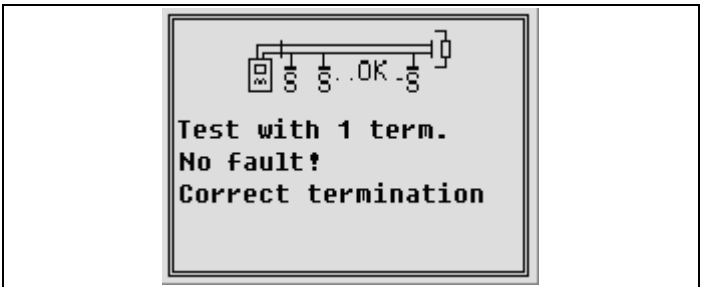
Figure 9: Screen after 'Test with 1 term.'
