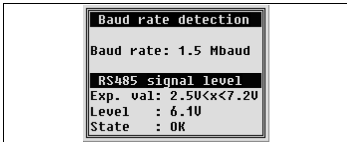
Figure 60: Baud rate detection
