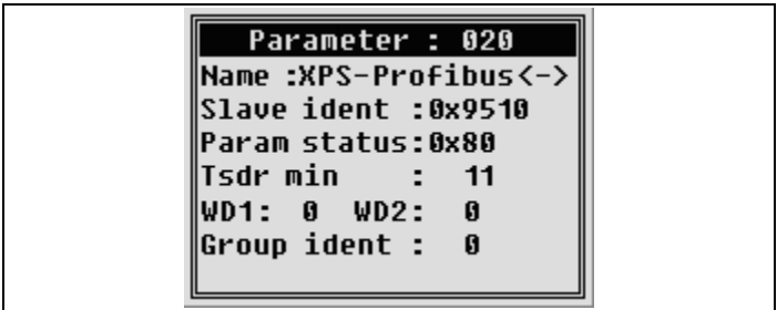
Figure 46: Entry mask 'Parameter'
