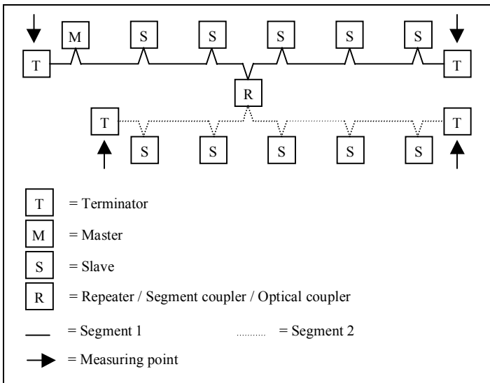
Figure 1: Connection NetTEST II in the cable thread
