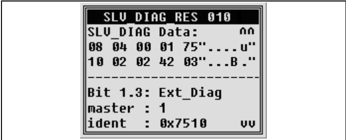
Figure 73: Screen 'Diagnostic event'
