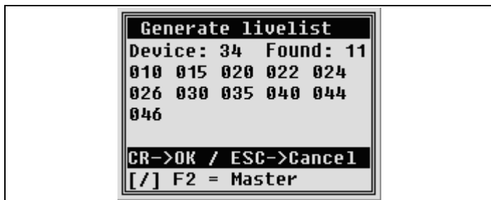
Figure 61: Generate Slave livelist
